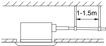
√ (Correct) 1/100 or more gradient
